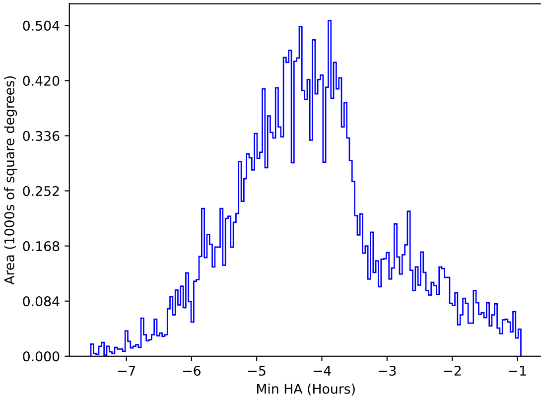
too_elab_r64_d2_giz_v3.4_10yrs All sky i band: Min HA
