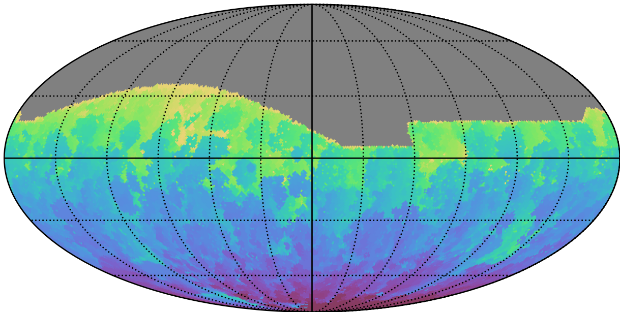
too_elab_r64_d2_giz_v3.4_10yrs All sky g band: Min HA
