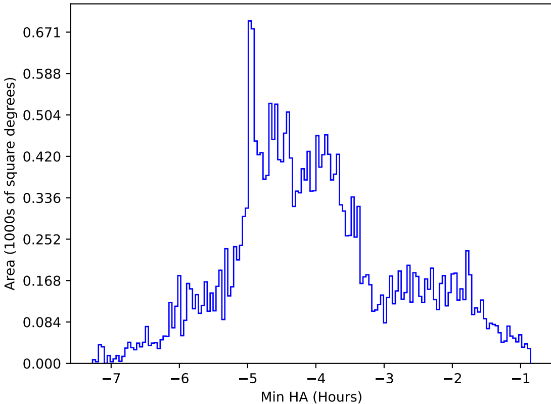
too_elab_r64_d2_giz_v3.4_10yrs All sky g band: Min HA
