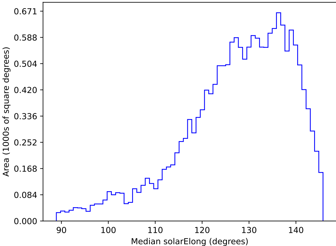
too_elab_r64_d2_giz_v3.4_10yrs WFD z band: Median solarElong
