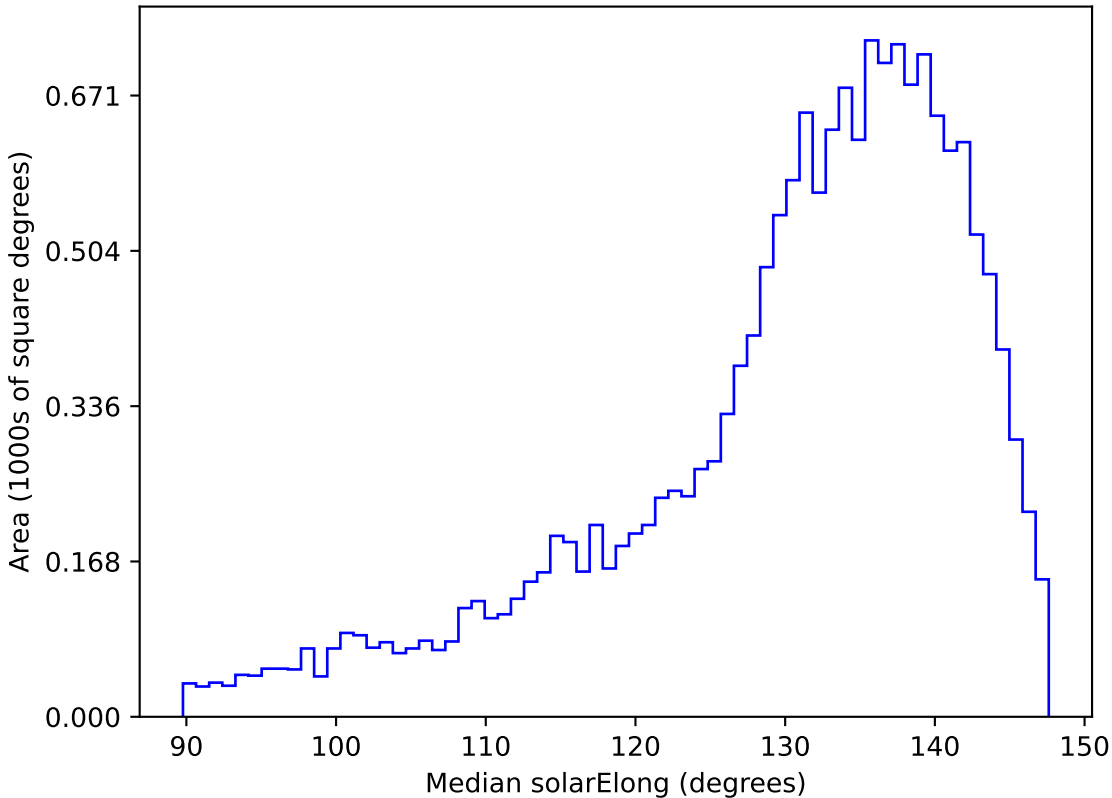
too_elab_r64_d2_giz_v3.4_10yrs WFD y band: Median solarElong
