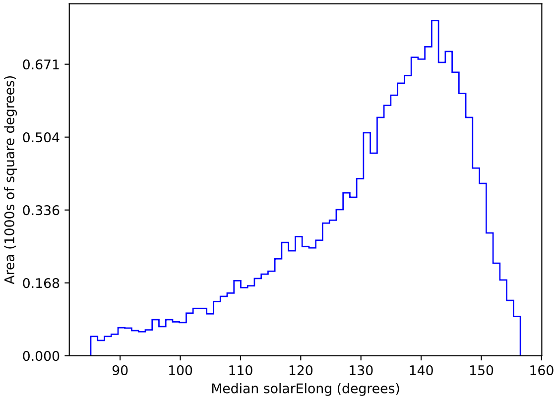
too_elab_r64_d2_giz_v3.4_10yrs WFD u band: Median solarElong
