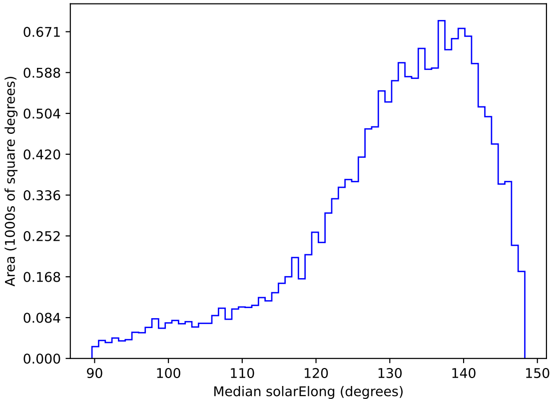
too_elab_r64_d2_giz_v3.4_10yrs WFD r band: Median solarElong
