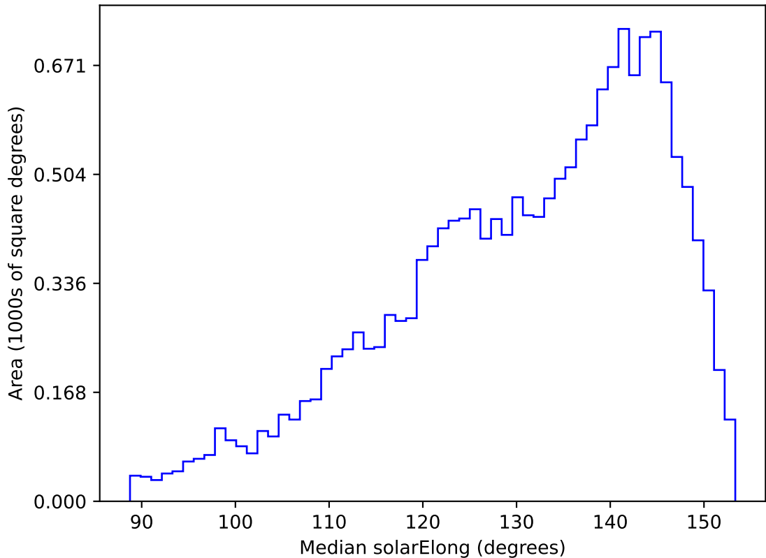
too_elab_r64_d2_giz_v3.4_10yrs WFD g band: Median solarElong
