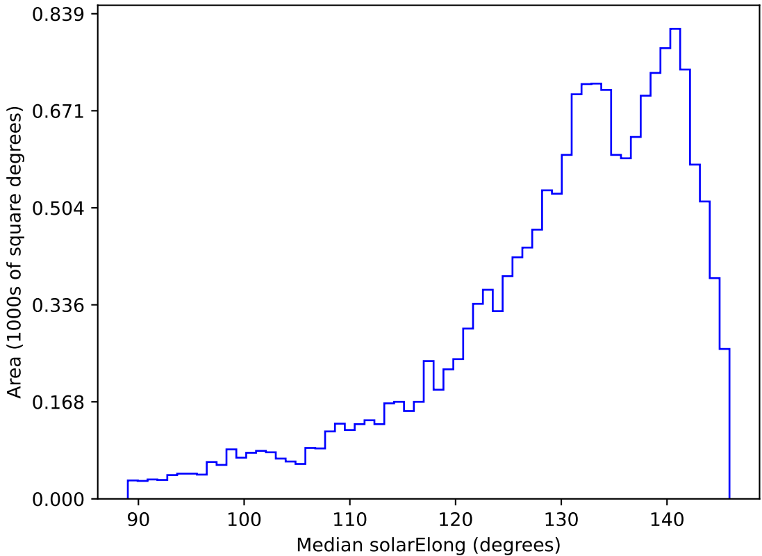
too_elab_r64_d2_giz_v3.4_10yrs WFD all bands: Median solarElong
