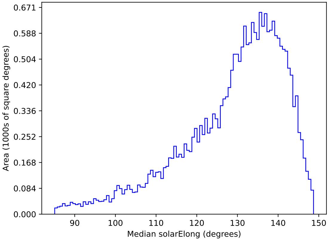
too_elab_r64_d2_giz_v3.4_10yrs All sky y band: Median solarElong
