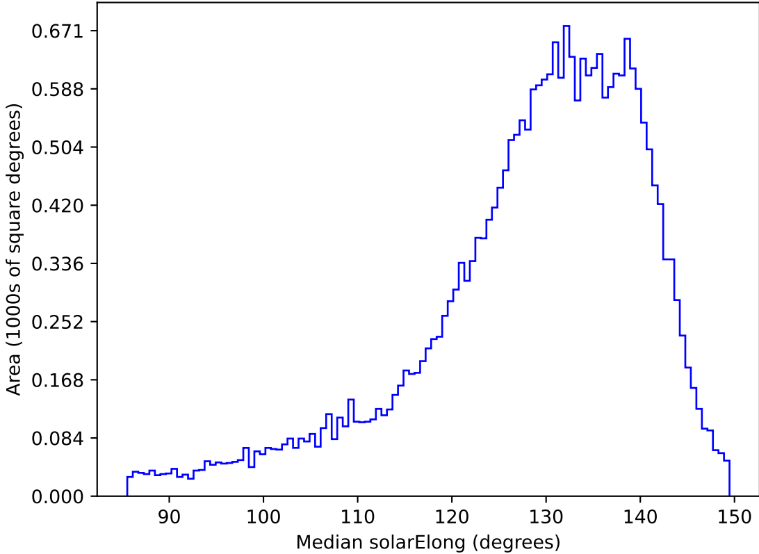
too_elab_r64_d2_giz_v3.4_10yrs All sky i band: Median solarElong
