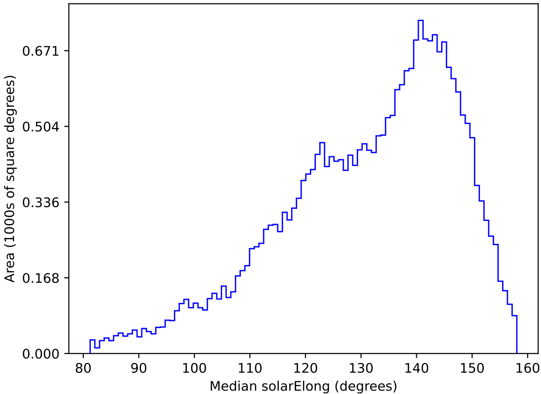
too_elab_r64_d2_giz_v3.4_10yrs All sky g band: Median solarElong
