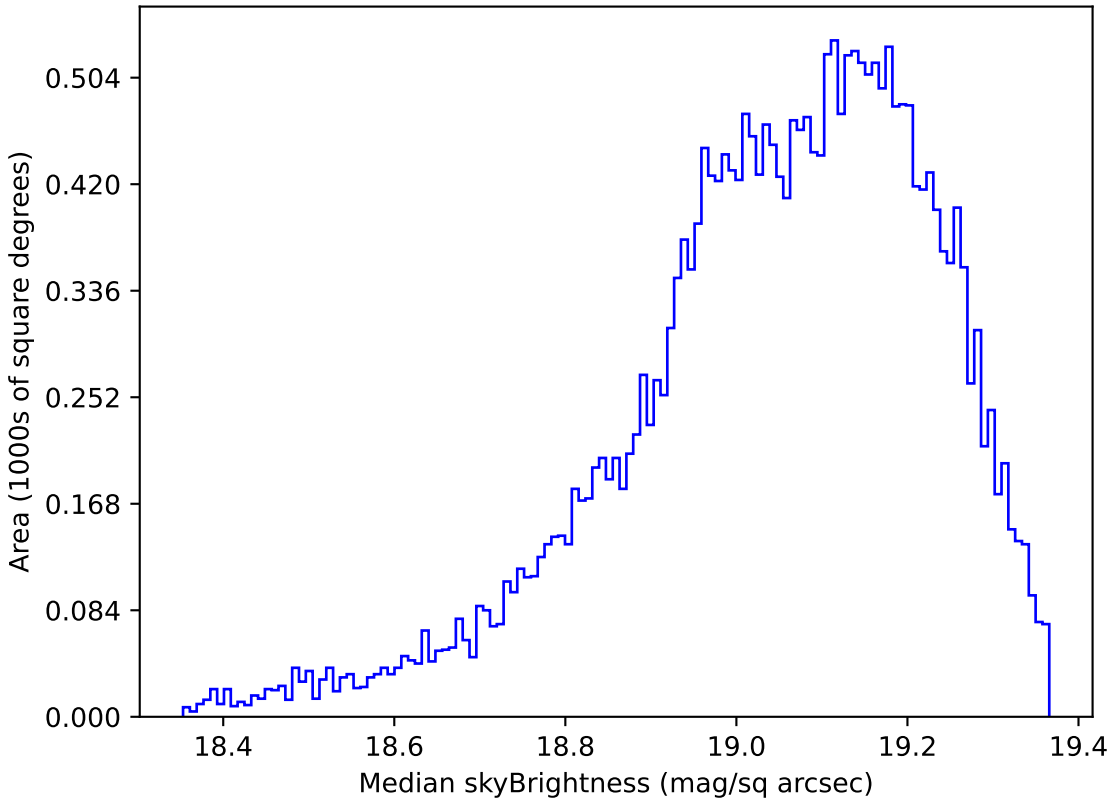
too_elab_r64_d2_giz_v3.4_10yrs Yr 1 z band: Median skyBrightness
