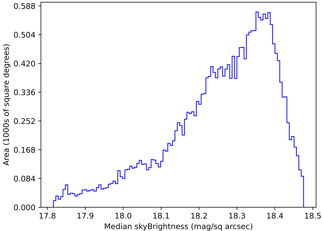
too_elab_r64_d2_giz_v3.4_10yrs Yr 1 y band: Median skyBrightness
