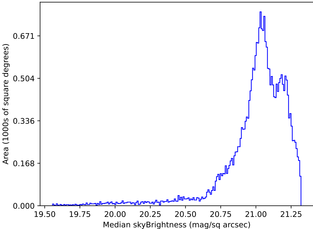
too_elab_r64_d2_giz_v3.4_10yrs Yr 1 r band: Median skyBrightness
