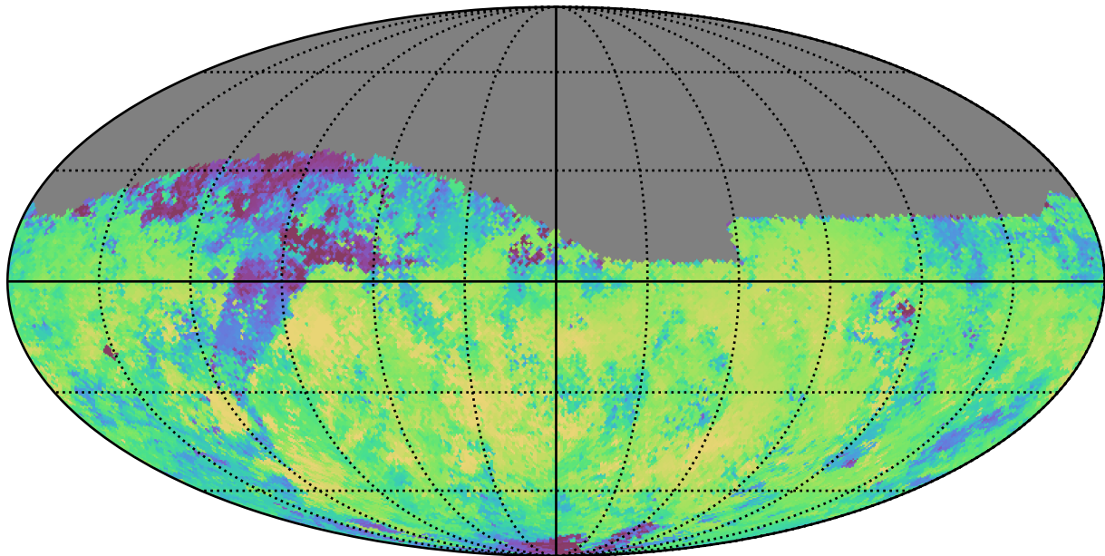
too_elab_r64_d2_giz_v3.4_10yrs Yr 1 i band: Median skyBrightness
