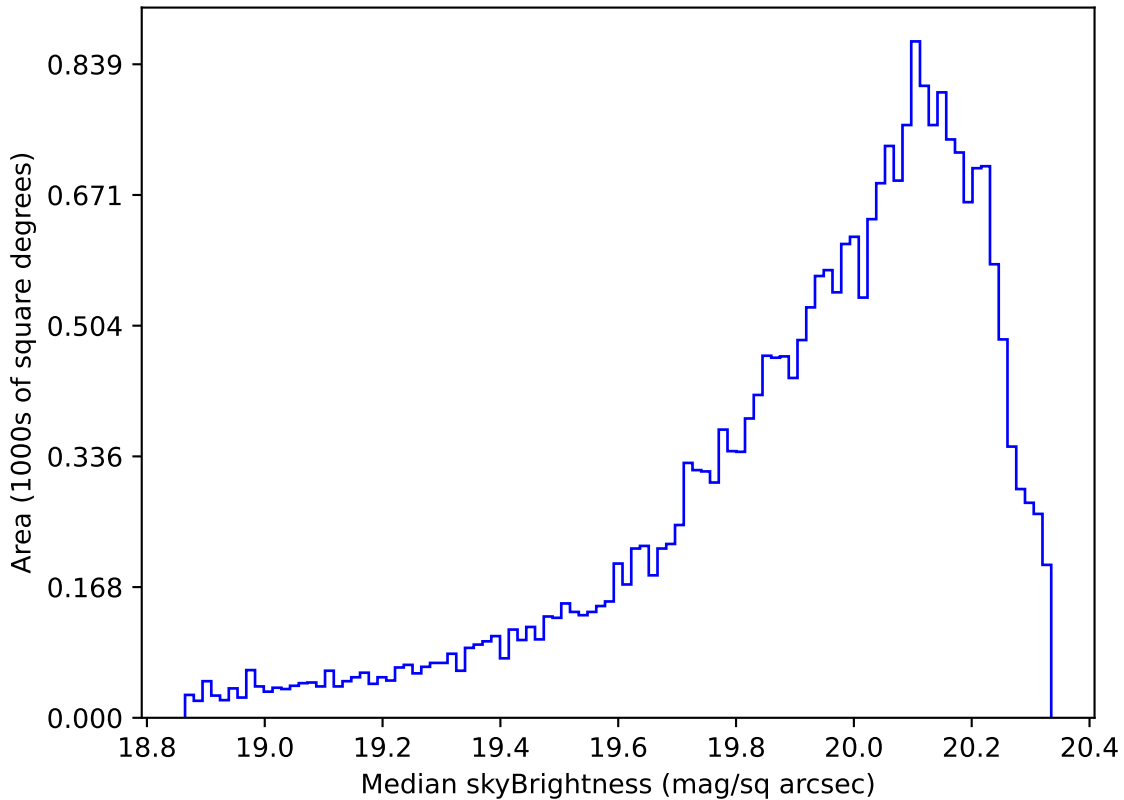
too_elab_r64_d2_giz_v3.4_10yrs Yr 1 i band: Median skyBrightness
