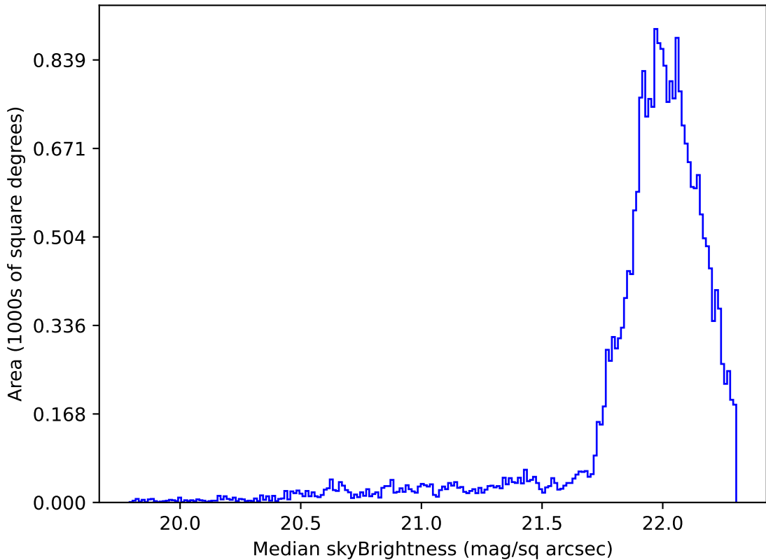
too_elab_r64_d2_giz_v3.4_10yrs Yr 1 g band: Median skyBrightness
