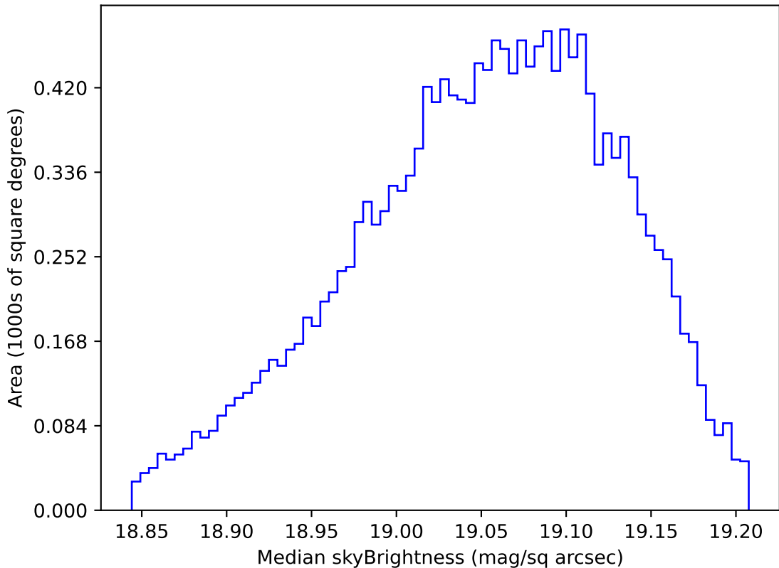
too_elab_r64_d2_giz_v3.4_10yrs WFD z band: Median skyBrightness
