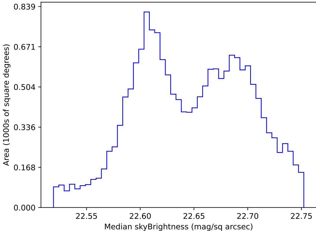
too_elab_r64_d2_giz_v3.4_10yrs WFD u band: Median skyBrightness
