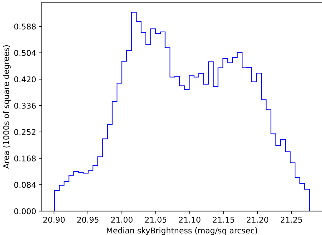
too_elab_r64_d2_giz_v3.4_10yrs WFD r band: Median skyBrightness
