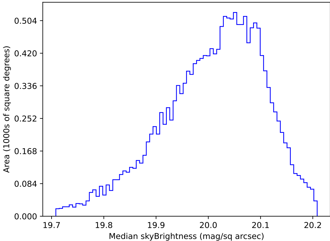
too_elab_r64_d2_giz_v3.4_10yrs WFD i band: Median skyBrightness
