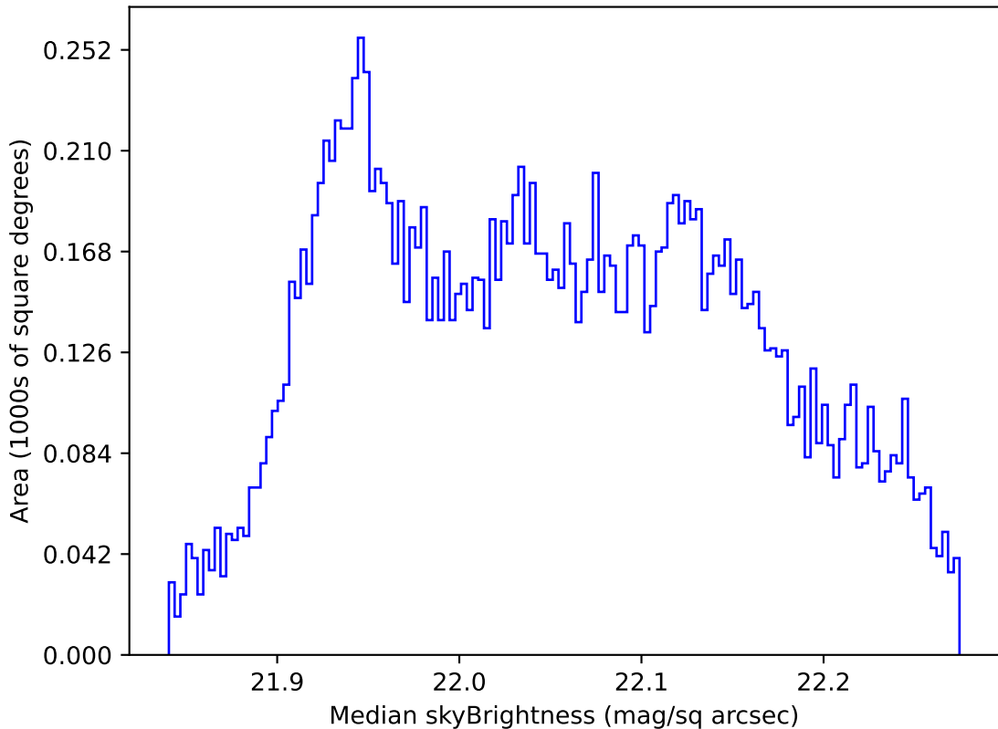
too_elab_r64_d2_giz_v3.4_10yrs WFD g band: Median skyBrightness
