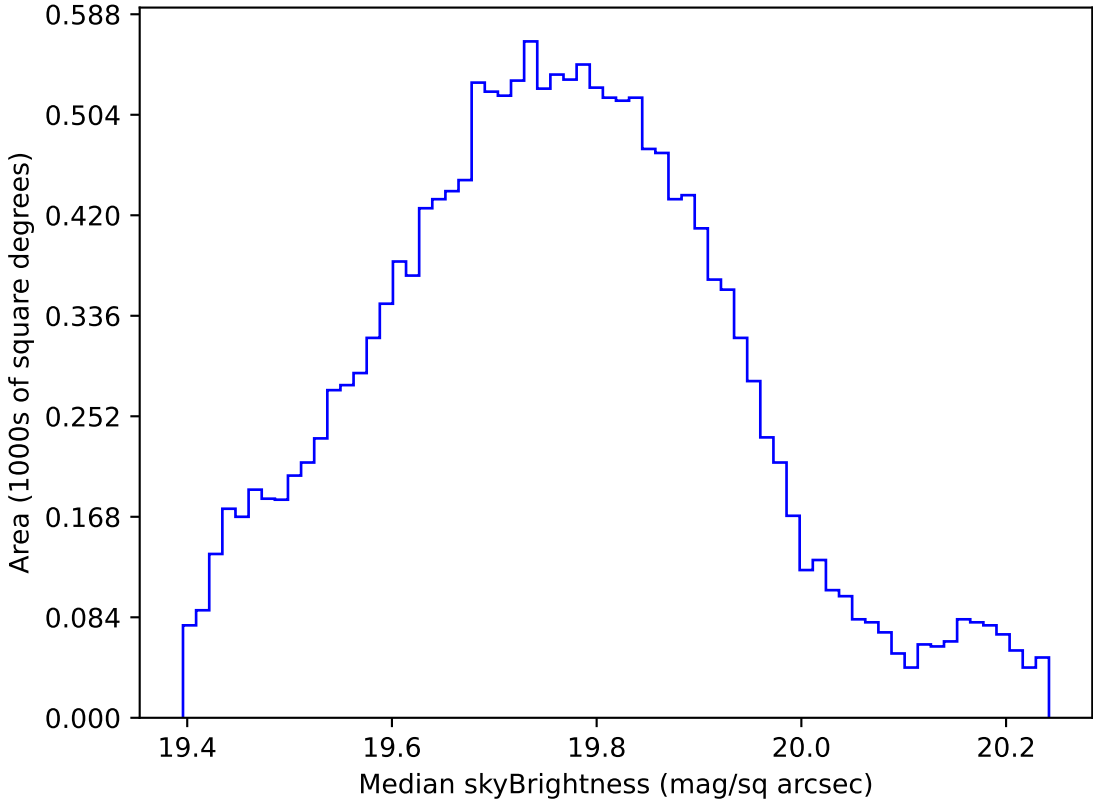
too_elab_r64_d2_giz_v3.4_10yrs WFD all bands: Median skyBrightness
