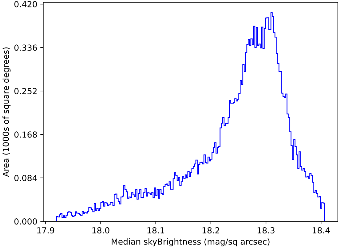
too_elab_r64_d2_giz_v3.4_10yrs All sky y band: Median skyBrightness
