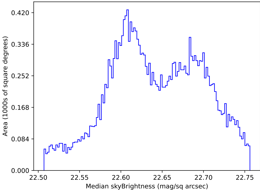
too_elab_r64_d2_giz_v3.4_10yrs All sky u band: Median skyBrightness
