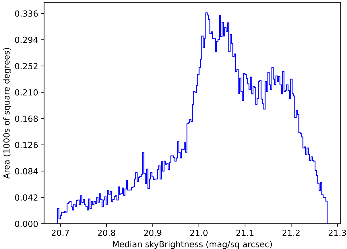
too_elab_r64_d2_giz_v3.4_10yrs All sky r band: Median skyBrightness
