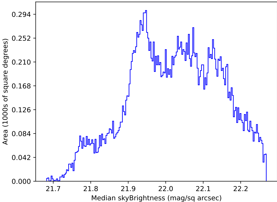
too_elab_r64_d2_giz_v3.4_10yrs All sky g band: Median skyBrightness
