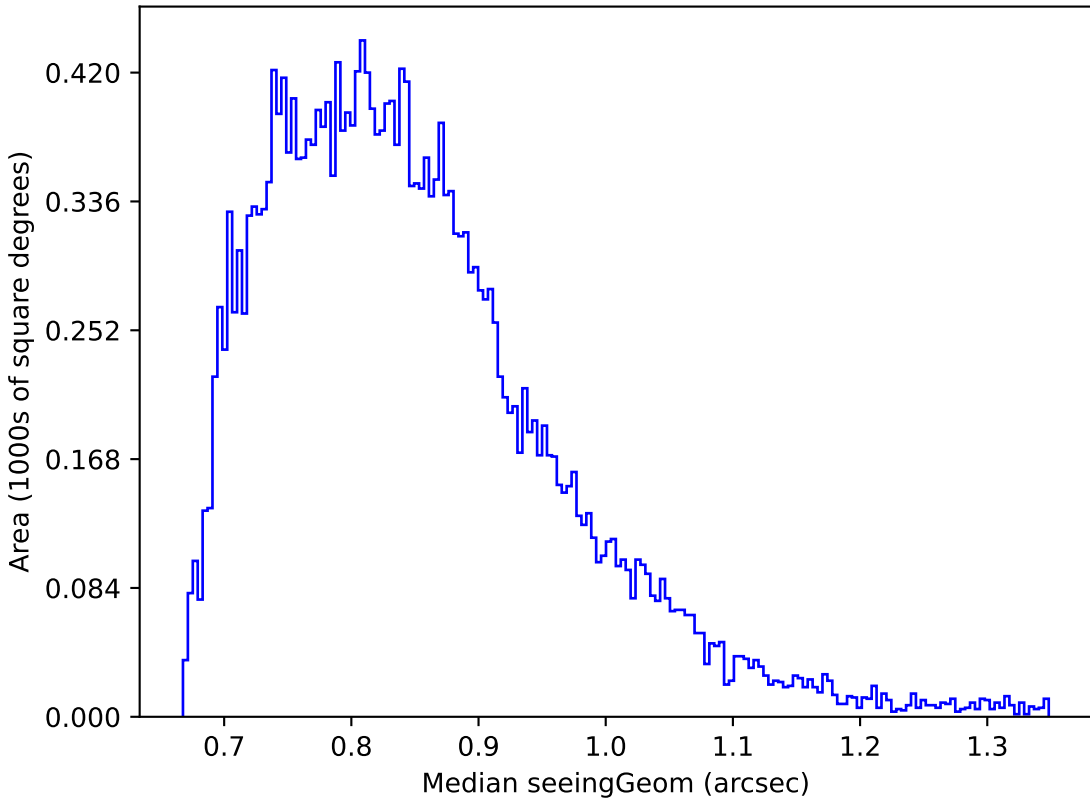
too_elab_r64_d2_giz_v3.4_10yrs Yr 1 z band: Median seeingGeom
