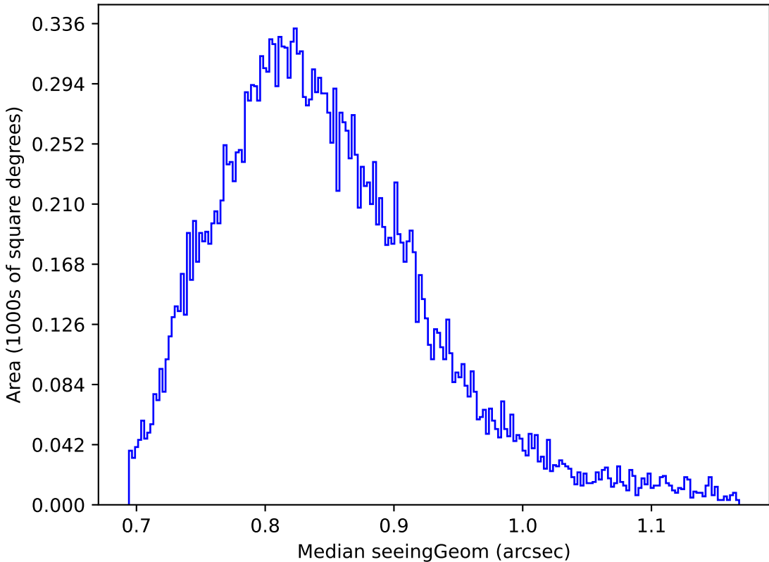
too_elab_r64_d2_giz_v3.4_10yrs Yr 1 y band: Median seeingGeom
