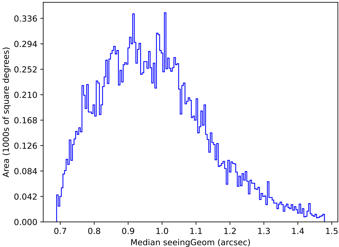
too_elab_r64_d2_giz_v3.4_10yrs Yr 1 u band: Median seeingGeom
