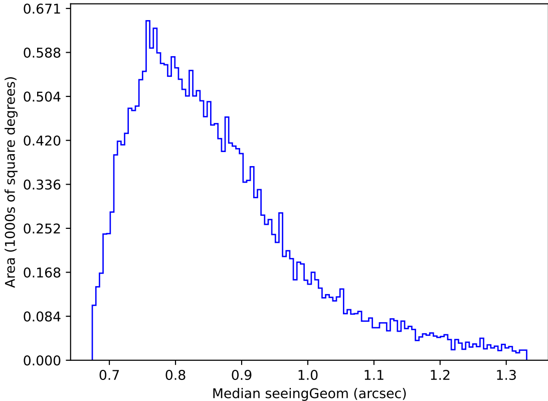
too_elab_r64_d2_giz_v3.4_10yrs Yr 1 r band: Median seeingGeom
