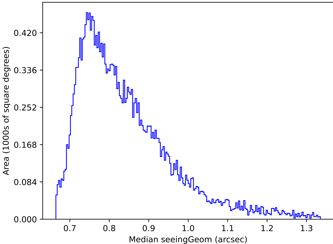
too_elab_r64_d2_giz_v3.4_10yrs Yr 1 i band: Median seeingGeom
