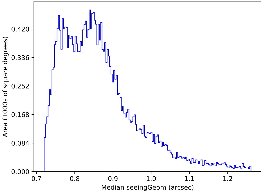
too_elab_r64_d2_giz_v3.4_10yrs Yr 1 all bands: Median seeingGeom
