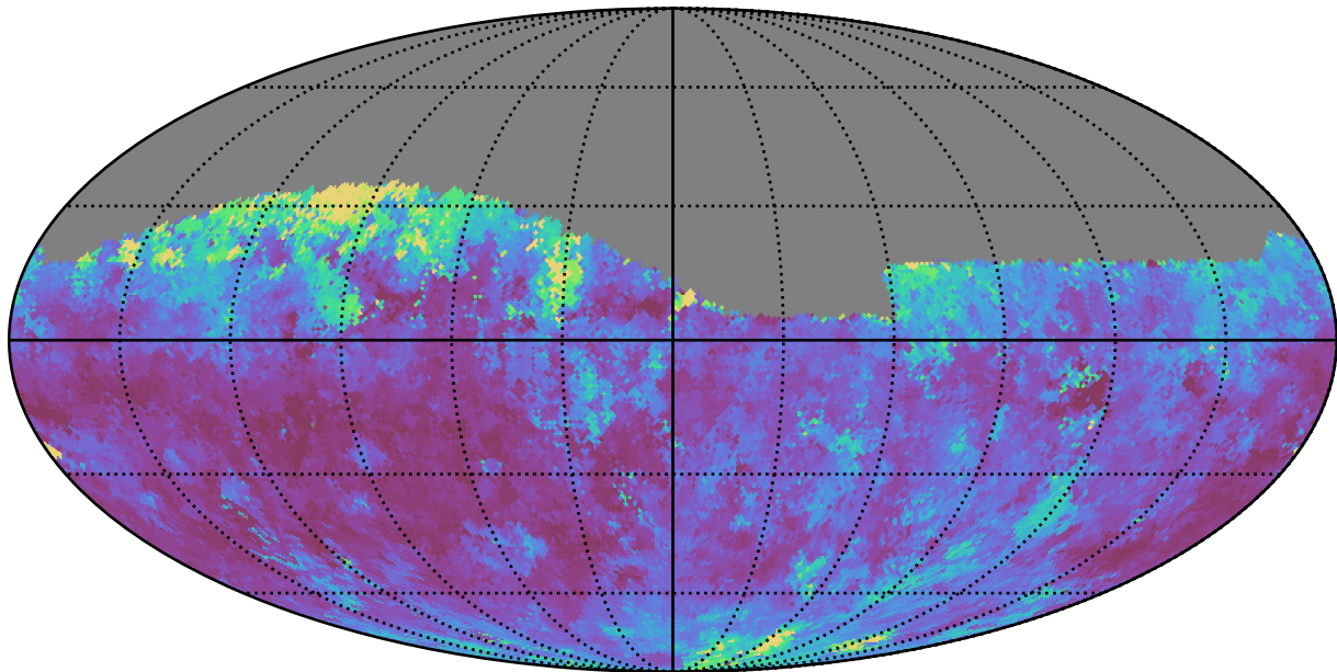
too_elab_r64_d2_giz_v3.4_10yrs Yr 1 z band: Median seeingEff
