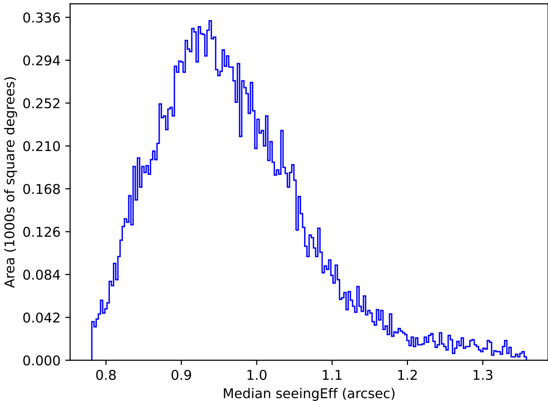
too_elab_r64_d2_giz_v3.4_10yrs Yr 1 y band: Median seeingEff
