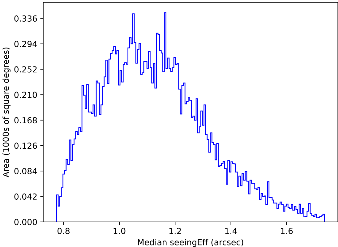
too_elab_r64_d2_giz_v3.4_10yrs Yr 1 u band: Median seeingEff
