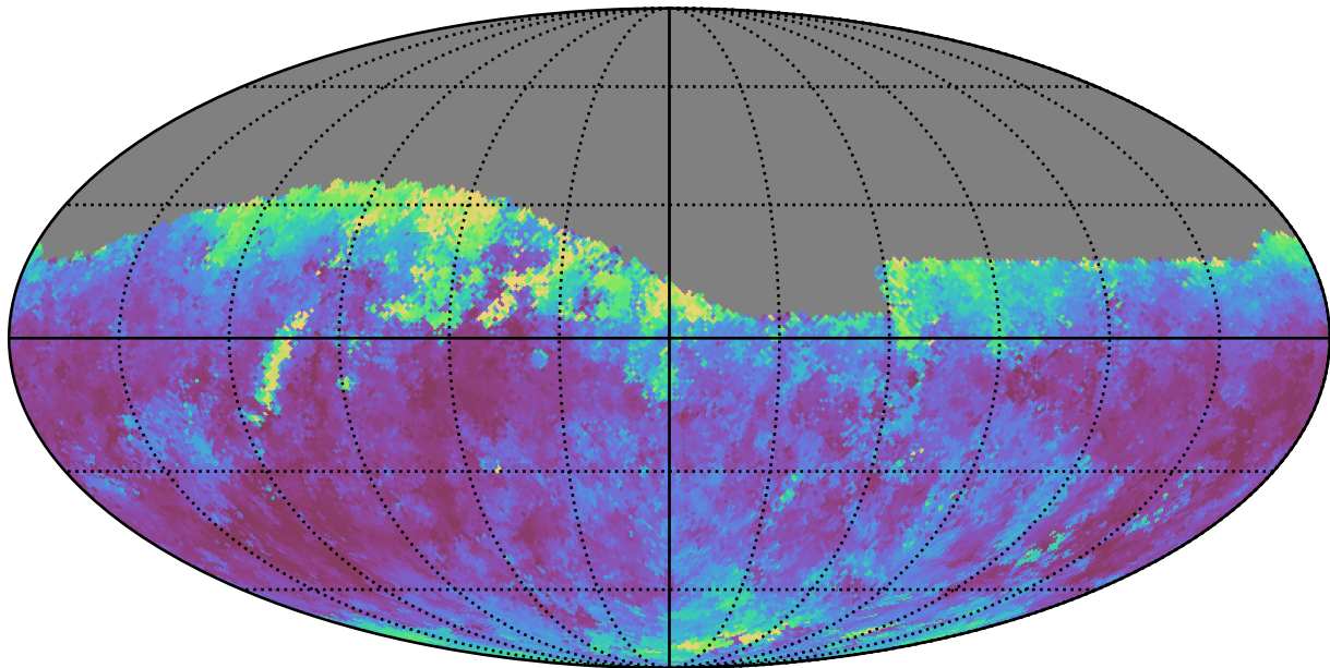
too_elab_r64_d2_giz_v3.4_10yrs Yr 1 r band: Median seeingEff
