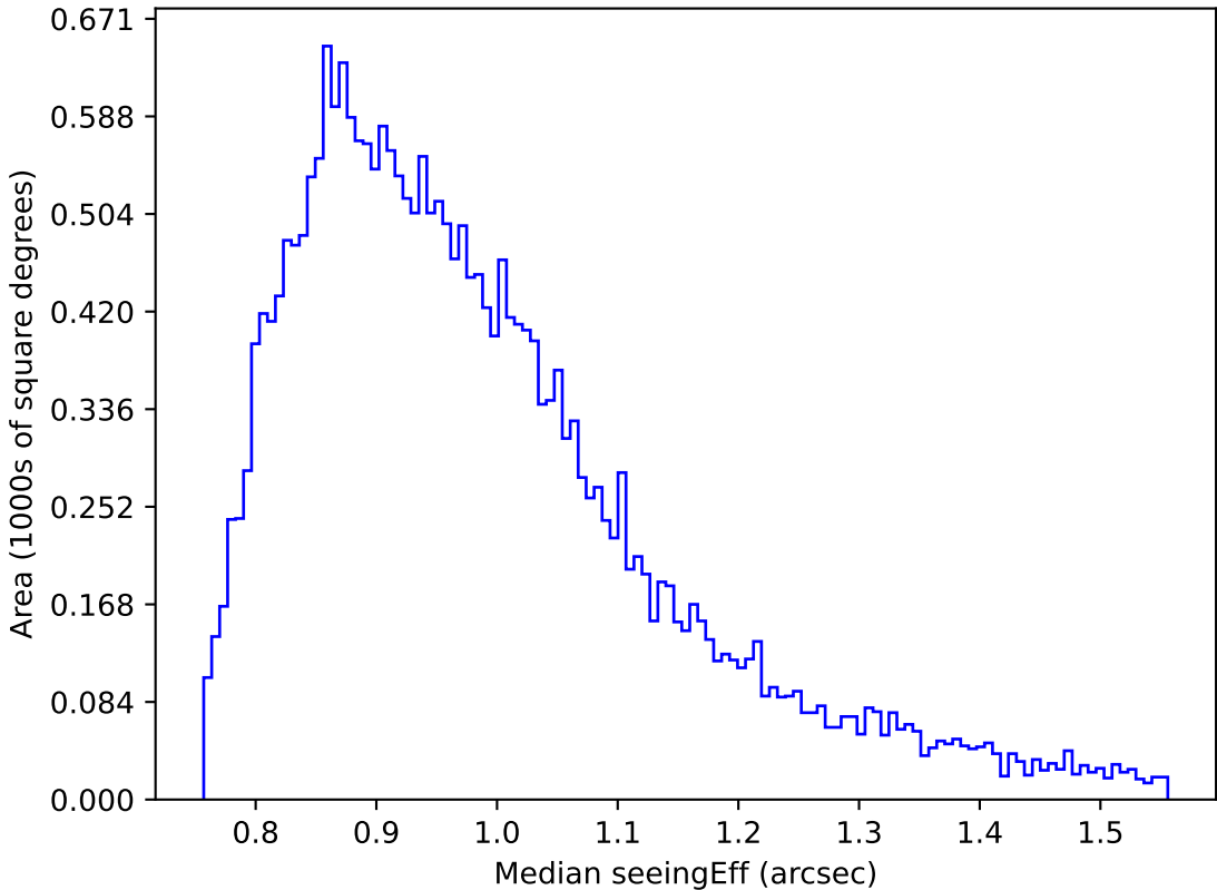
too_elab_r64_d2_giz_v3.4_10yrs Yr 1 r band: Median seeingEff
