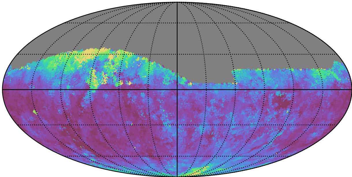
too_elab_r64_d2_giz_v3.4_10yrs Yr 1 i band: Median seeingEff
