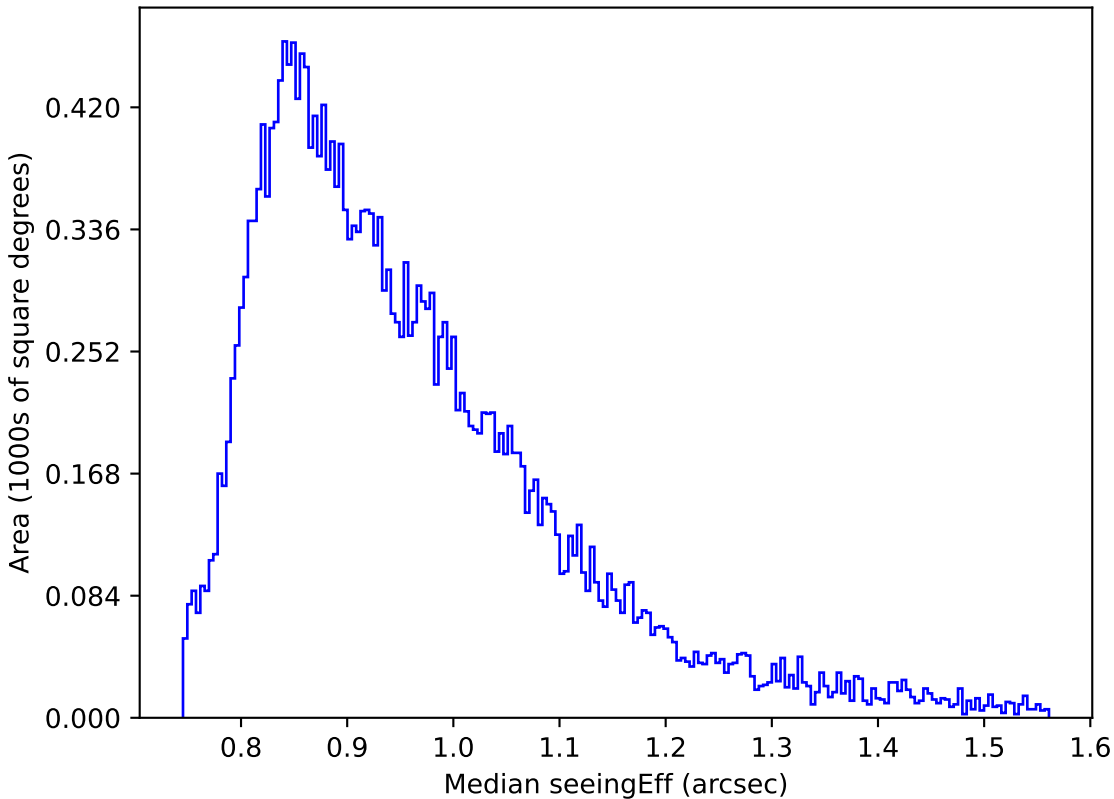
too_elab_r64_d2_giz_v3.4_10yrs Yr 1 i band: Median seeingEff
