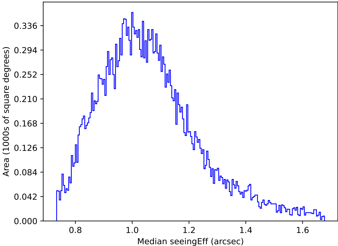
too_elab_r64_d2_giz_v3.4_10yrs Yr 1 g band: Median seeingEff
