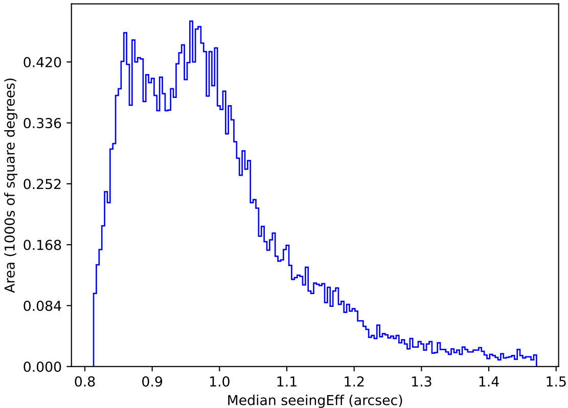
too_elab_r64_d2_giz_v3.4_10yrs Yr 1 all bands: Median seeingEff
