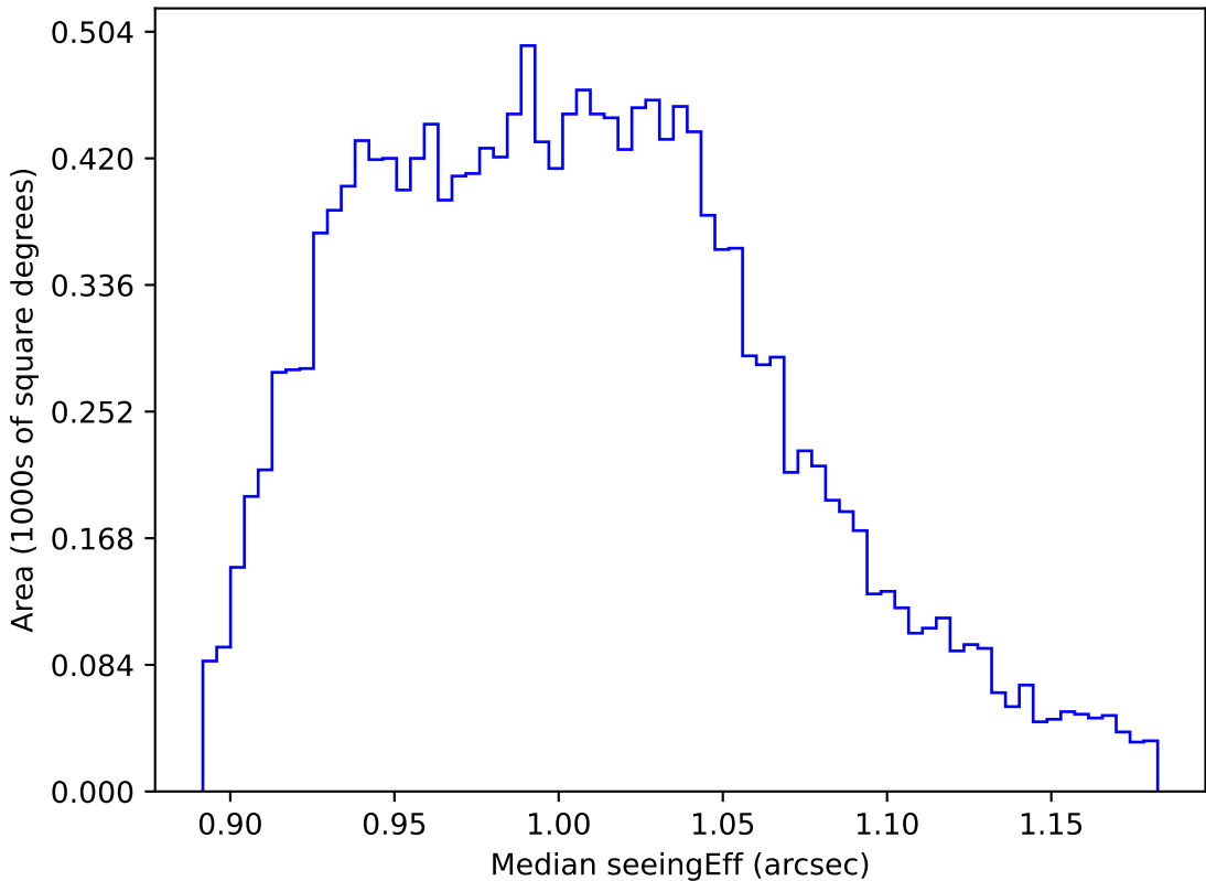
too_elab_r64_d2_giz_v3.4_10yrs WFD y band: Median seeingEff
