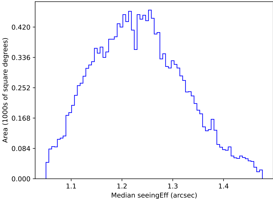
too_elab_r64_d2_giz_v3.4_10yrs WFD u band: Median seeingEff
