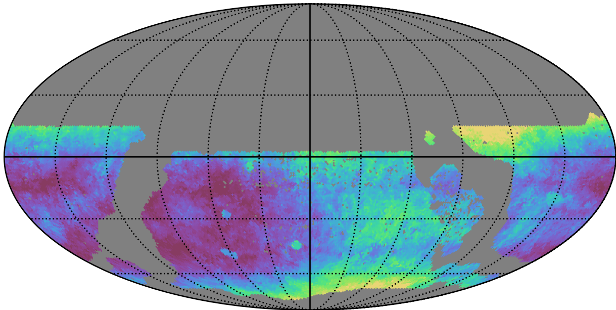
too_elab_r64_d2_giz_v3.4_10yrs WFD r band: Median seeingEff
