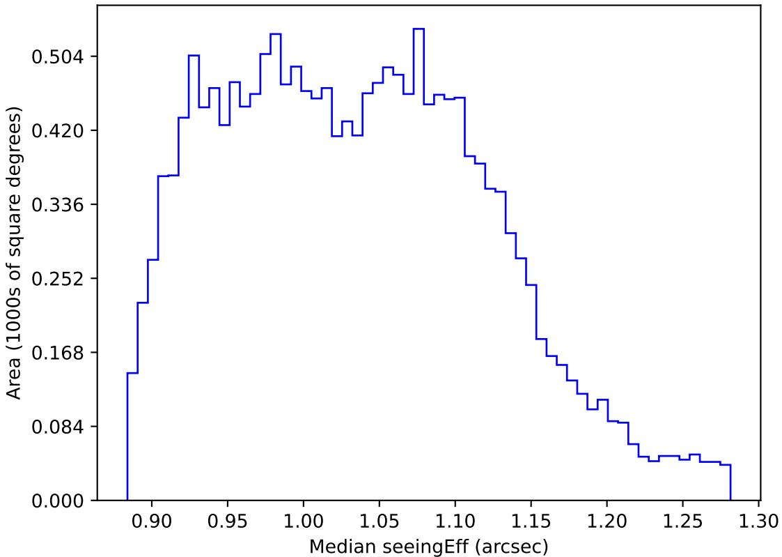
too_elab_r64_d2_giz_v3.4_10yrs WFD r band: Median seeingEff
