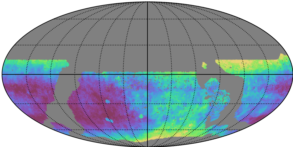
too_elab_r64_d2_giz_v3.4_10yrs WFD i band: Median seeingEff
