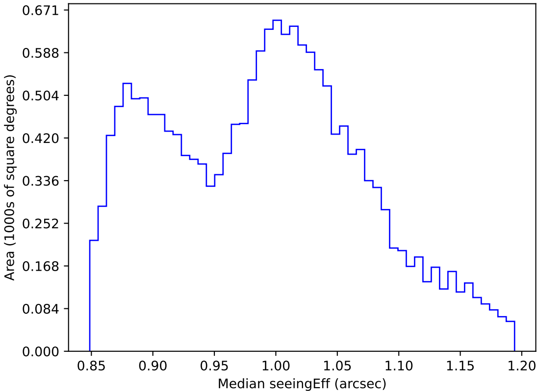
too_elab_r64_d2_giz_v3.4_10yrs WFD i band: Median seeingEff
