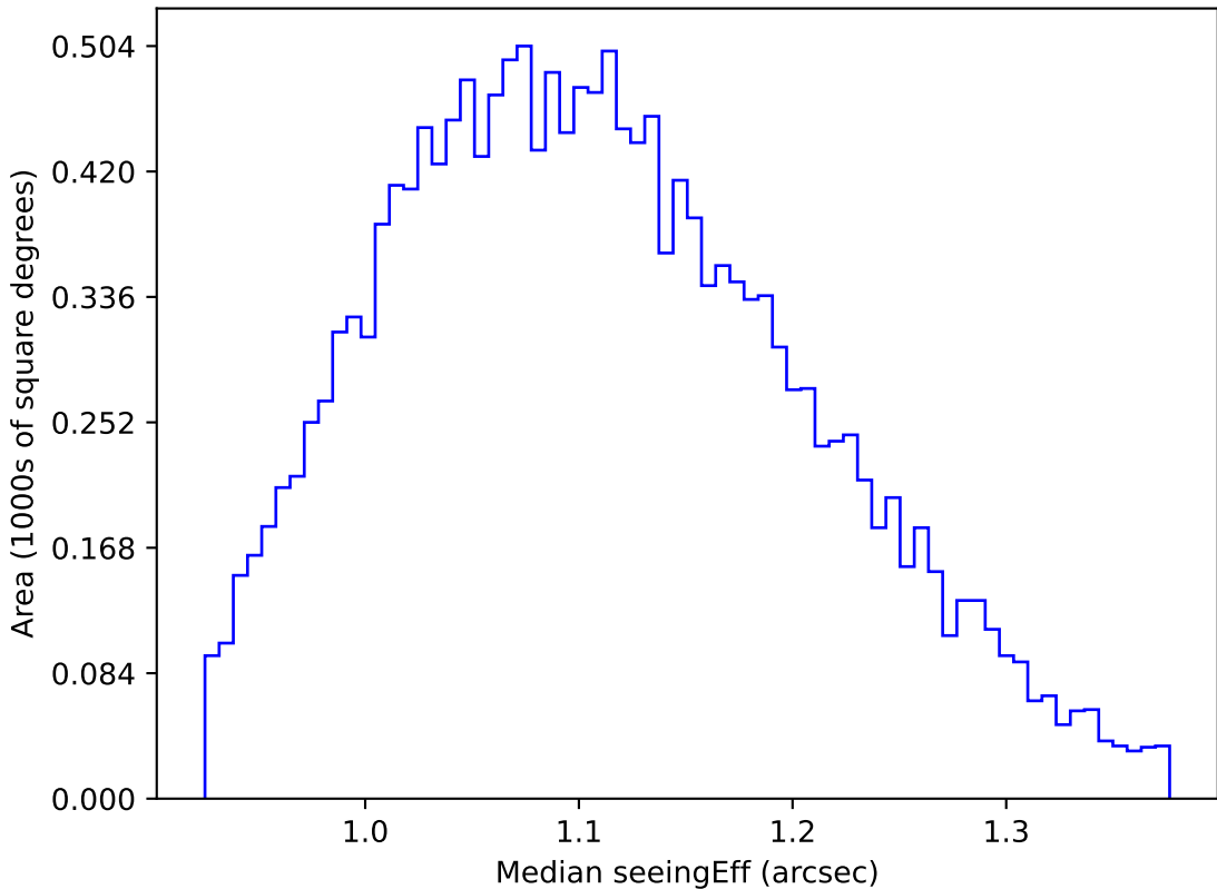
too_elab_r64_d2_giz_v3.4_10yrs WFD g band: Median seeingEff
